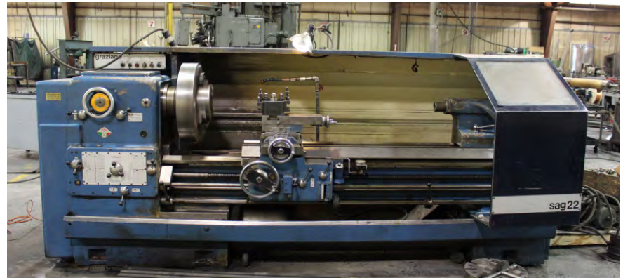
POLAMCO TUR 63-A, 5.5" HOLLOW SPINDLE, 24" X 108" CC, 20" 4 JAW CHUCK, 18" 3 JAW CHUCK, TAPER ATTACHMENT, STEADY REST, S/N 0381-42-146
